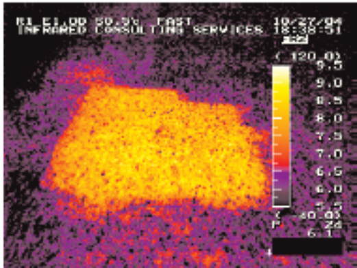
Infrared Scanning Locates and Defines the Wet insulation
